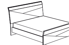
KING SIZE BED PJCA0175CN Inner size inch 76 3/4" x 81 1/2" cm 195 x 207 inch W 85" D 92" H 53" cm L 216 P 231 H 134 Crts 3 kg 132,5 m 3 0,456
